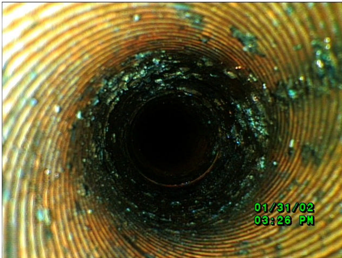
Source: Chemical, Inc. Fiberoptic Scoping reveals severe deposition and corrosion.
